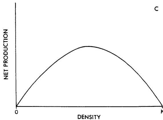
Fig. 2. Interactions of population density, production, and growth.
