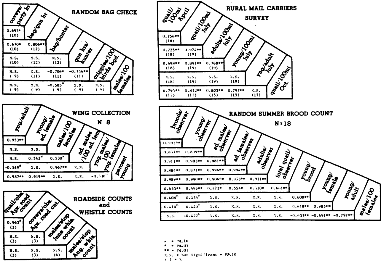
Fig. 1. Correlation coefficients (r) between indices of selected population and harvest surveys in Kansas, 1961-1980.
