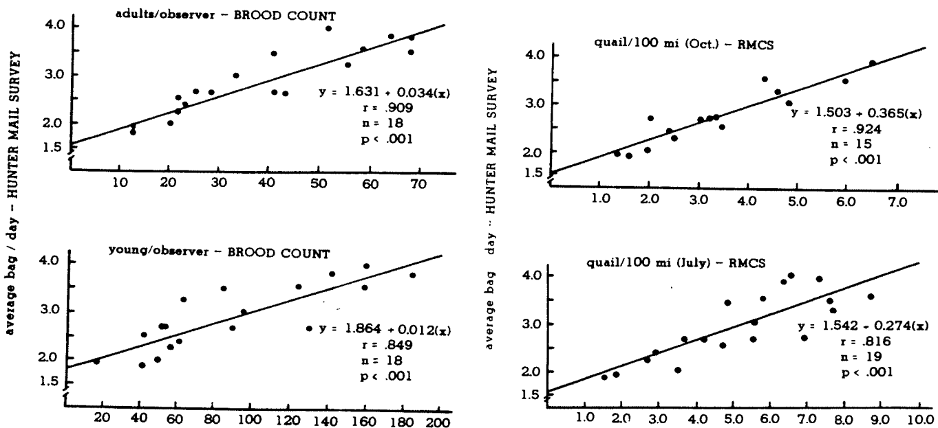
Fig. 2. Relationships of selected random summer brood count and rural mail carrier survey indices to the mail harvest survey index average bag/day in Kansas, 1962-1980.
