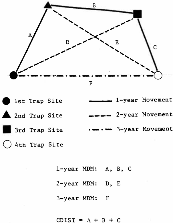
Fig. 2. Diagram and description of the various distances calculated for a quail captured four consecutive winters.
