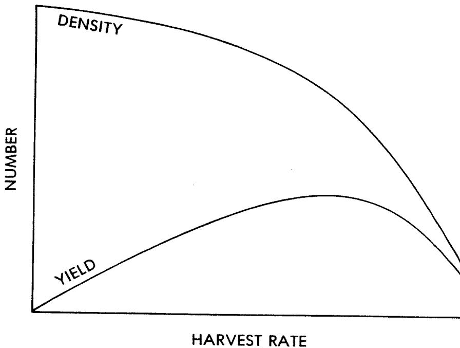
Fig. 3. Relationship of harvest rate to standing density and sustained yield.
