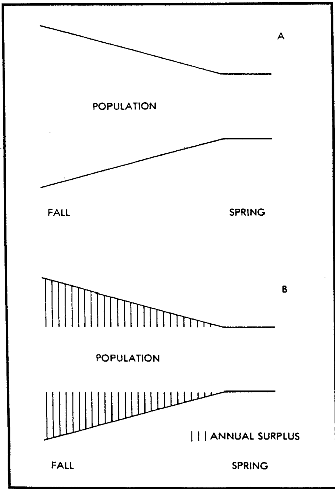
Fig. 1. Traditional view of an "annual surplus".
