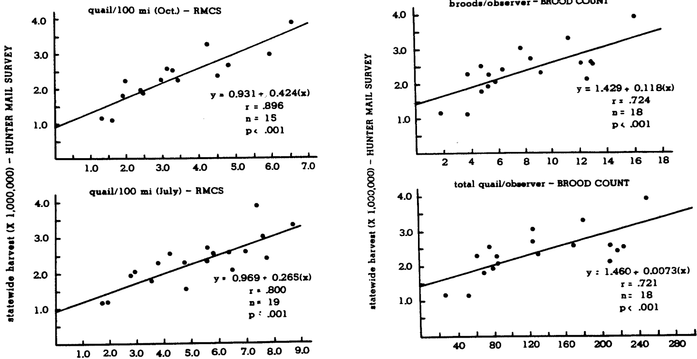
Fig. 3. Relationships of selected random summer brood count and rural mail carrier survey indices to the mail harvest survey index statewide (total) harvest in Kansas, 1962-1980.
