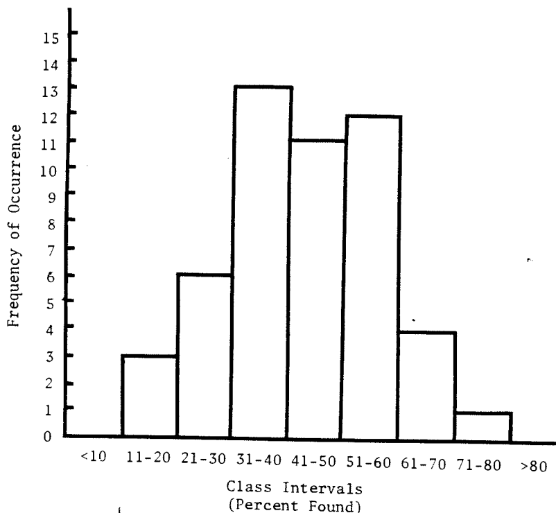
Fig. 1. Frequency distribution of the percentage of bobwhites found by hunters.
